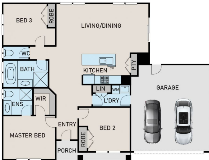
FLOOR PLAN
