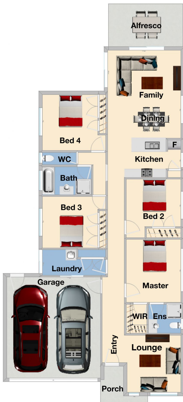
Floor Plan
