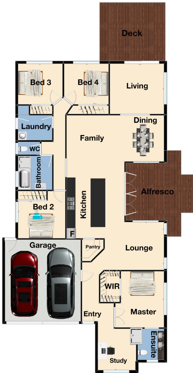
Floor Plan
